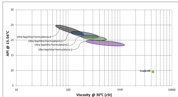
UltraNaphtha® Test Results Using a 7.4API Super Heavy Crude
